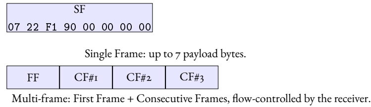
Figure 2.2.: ISO 15765-2 (ISO-TP) protocol data units. Short diagnostic messages fit in a Single Frame; longer responses use First Frame + Consecutive Frames with Flow Control.
