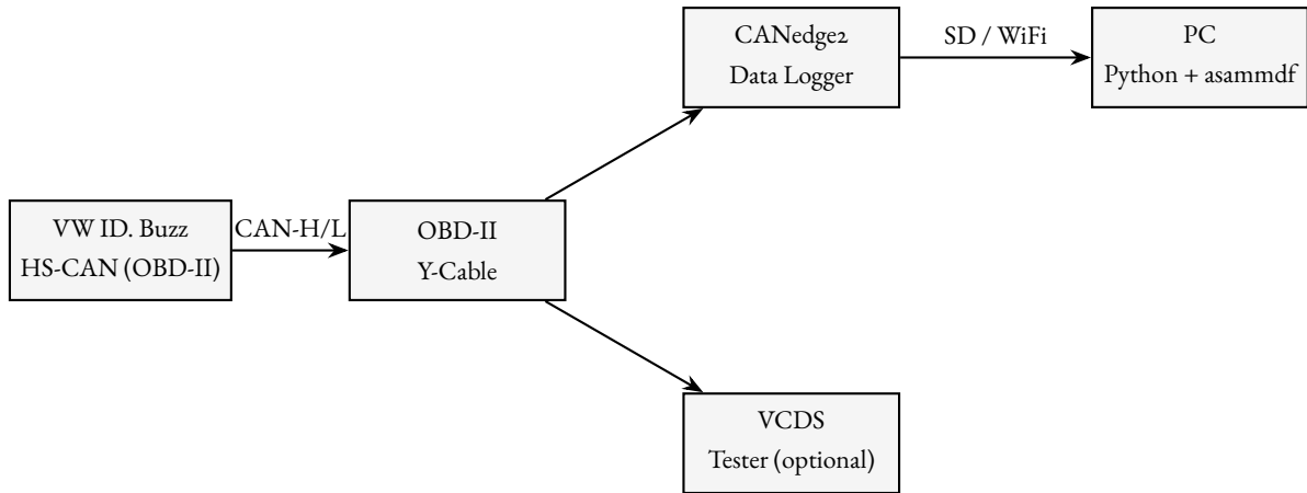
Figure 3.1.: Overall measurement setup. The CANedge2 logger is powered by the vehicle via the OBD-II Y-cable and writes MDF4 files to its SD card for offline analysis on the PC.
